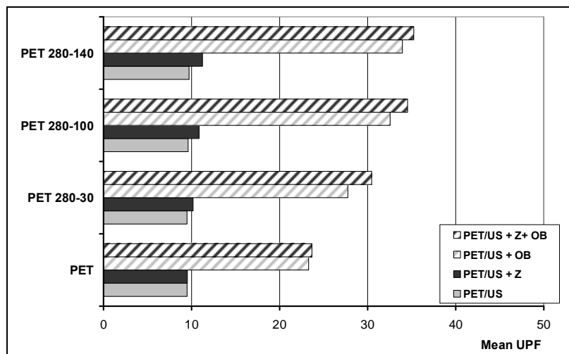
Figure 5 UV protection expressed through mean UPF of PET fabrics after ultrasound treatment and optical brightening
