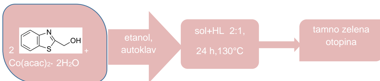
Schema 2. Prikaz sinteze \text{Co}(\text{acac})_2 \cdot 2\text{H}_2\text{O} i HL u molarnom omjeru 2:1
