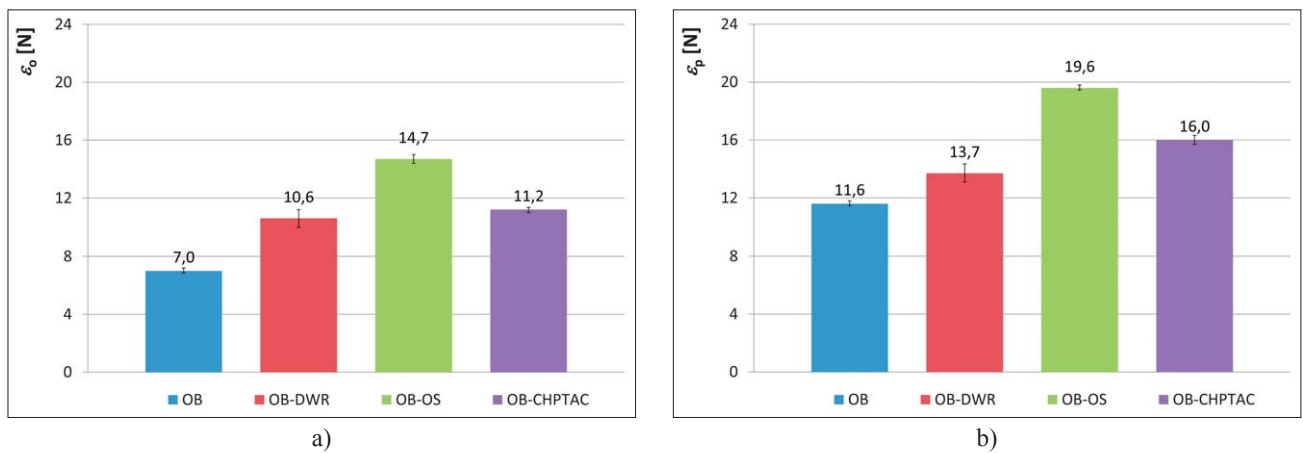
Fig.3 Breaking elongation of optical brightened waste cotton fabric before and after cationization: a) warp direction (ε 0 ), and b) weft direction (ε p )
