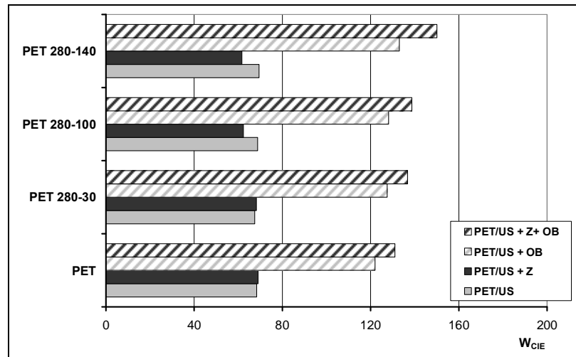
Figure 4 Absorption of optical brightener (OB) expressed through CIE whiteness ( W_{CIE} ) of PET fabrics
