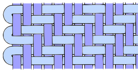
Sl. 11. Keper vez (2/2) [22]
