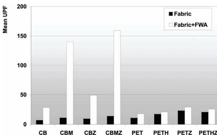
Figure 4. Mean UPF values of cotton and polyester fabrics after surface modification and treatment with zeolite and FWA's.
